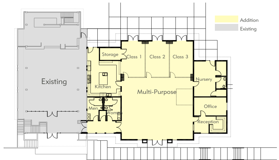
Floor Plan
